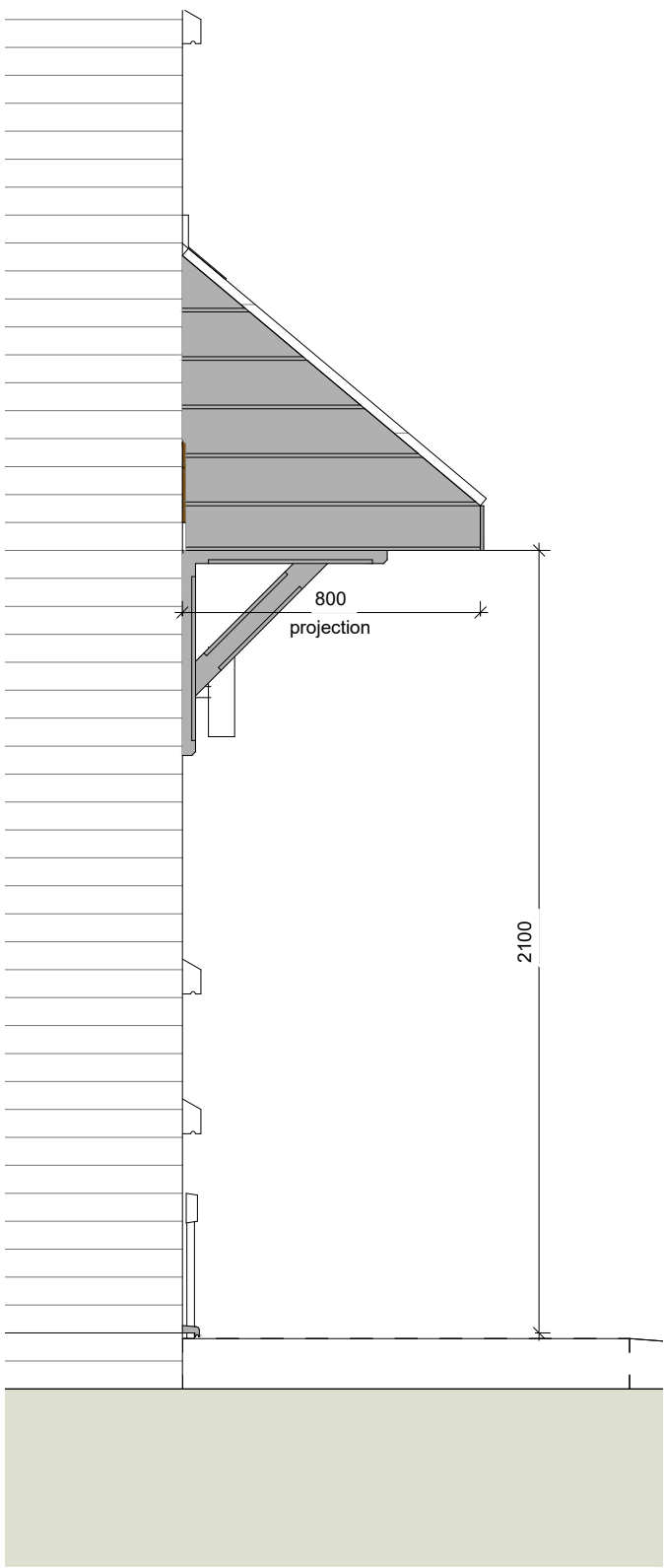
2 Gable Elevation 1 : 20
